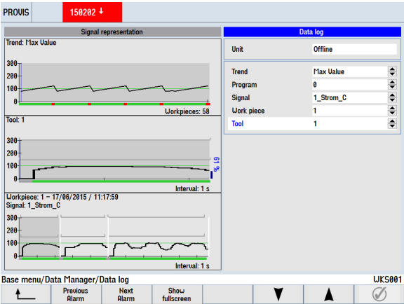
User interface integrated on machine control
