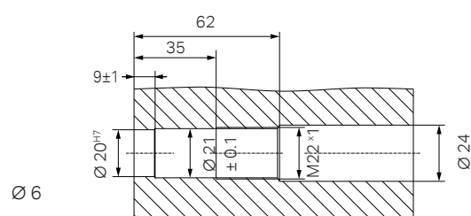
Example of dowel hole and fitting
